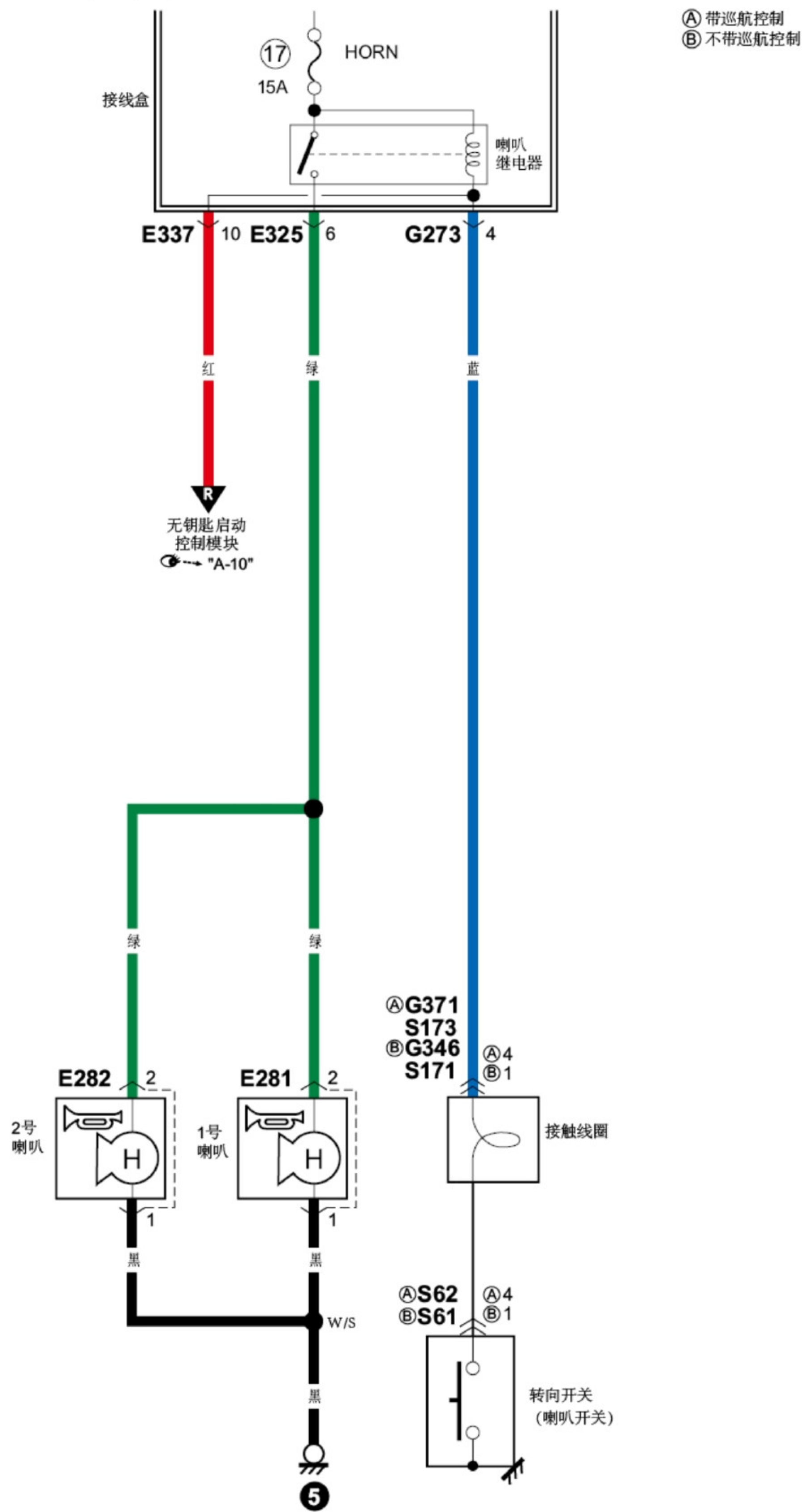
B-7喇叭电路图 AENDAA0A910E017 (10 (01))
